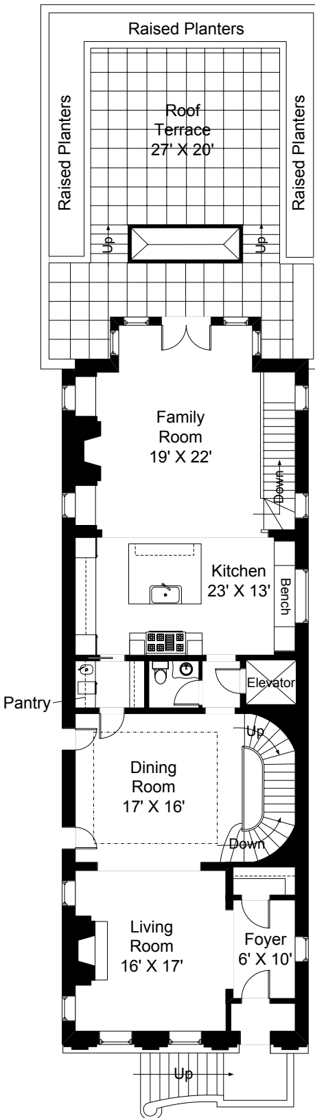
MAIN LEVEL
